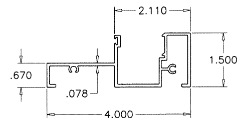
3 STD. THRESHOLD
