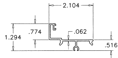
12 SIDELITE TOP/BOTTOM ADAPTER
