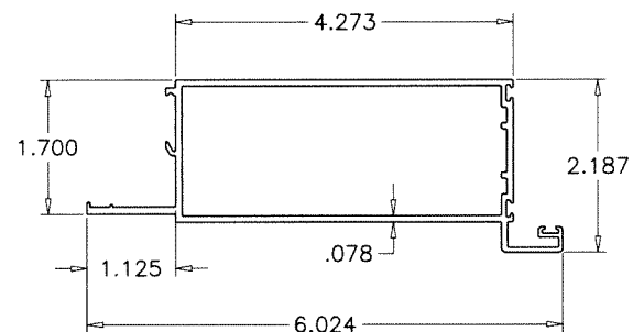
7 ASTRAGAL STILE (ACTIVE)
