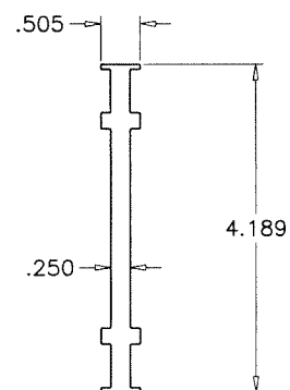
13 MULLION
