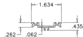
10 W'STRIP ADAPTER
