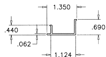
5 FRAME COVER
