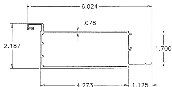
8 ASTRAGAL STILE (INACTIVE)
