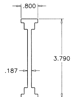
32 SIDELITE REINF.
