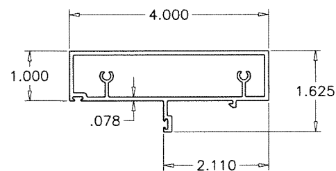
1 FRAME HEAD
