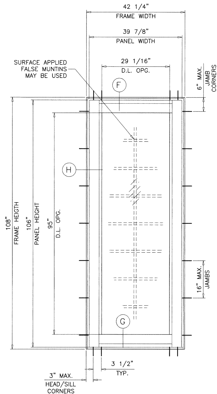
TYPICAL ELEVATION ( O )
